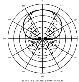
Polar Pattern
