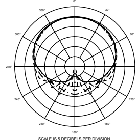
Polar Pattern
