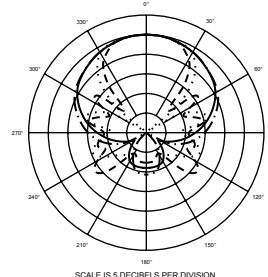
Polar Pattern
