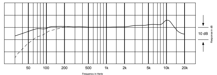
Frequency Response
