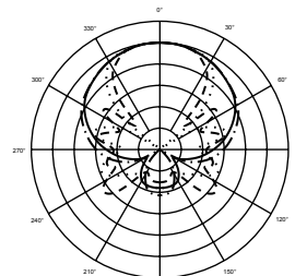
Polar Pattern
